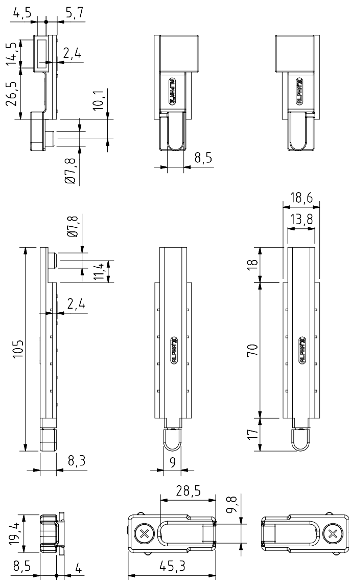
Ponteira afinável # Tuning tip # Ferrule regulable # Bague réglable
